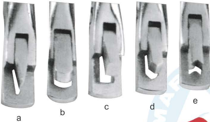
MI-143 Ear Notcher S.S. Design in the Center of the ear
